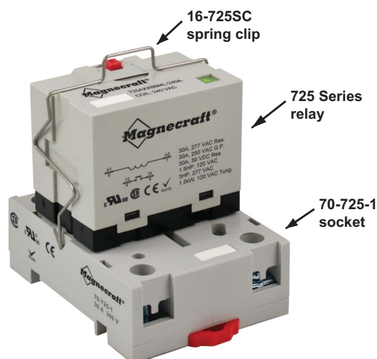
Relay Mounting Example:
